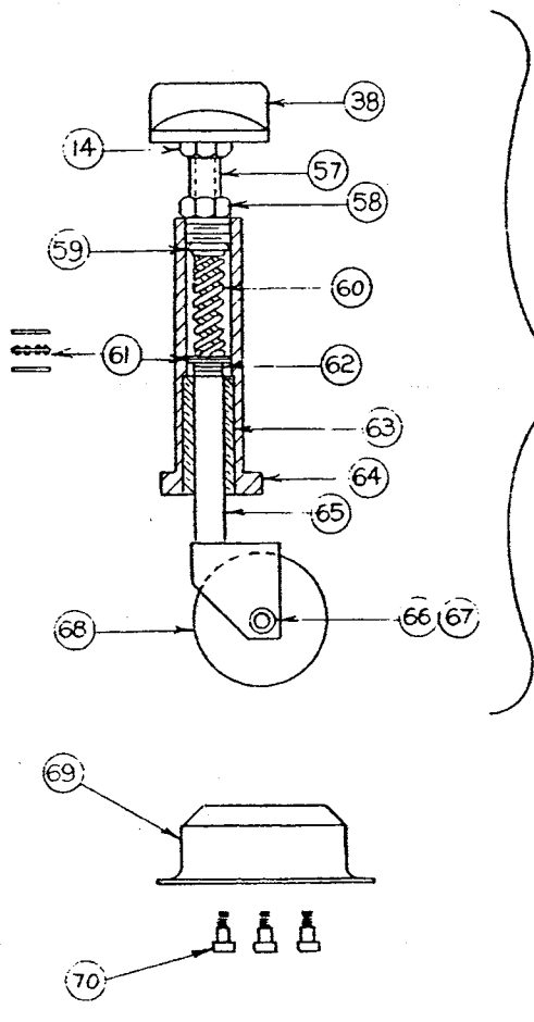
832477 Caster Tube Asm.
